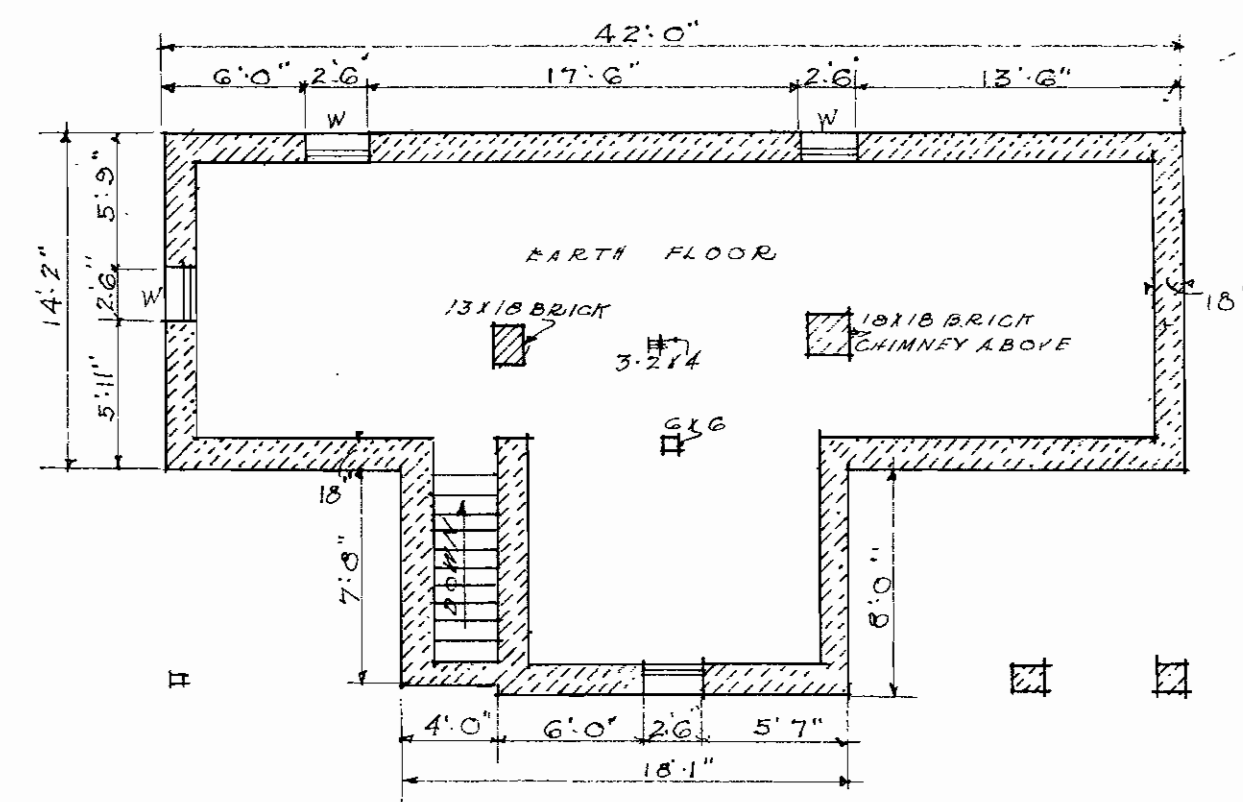
BASEMENT PLAN
