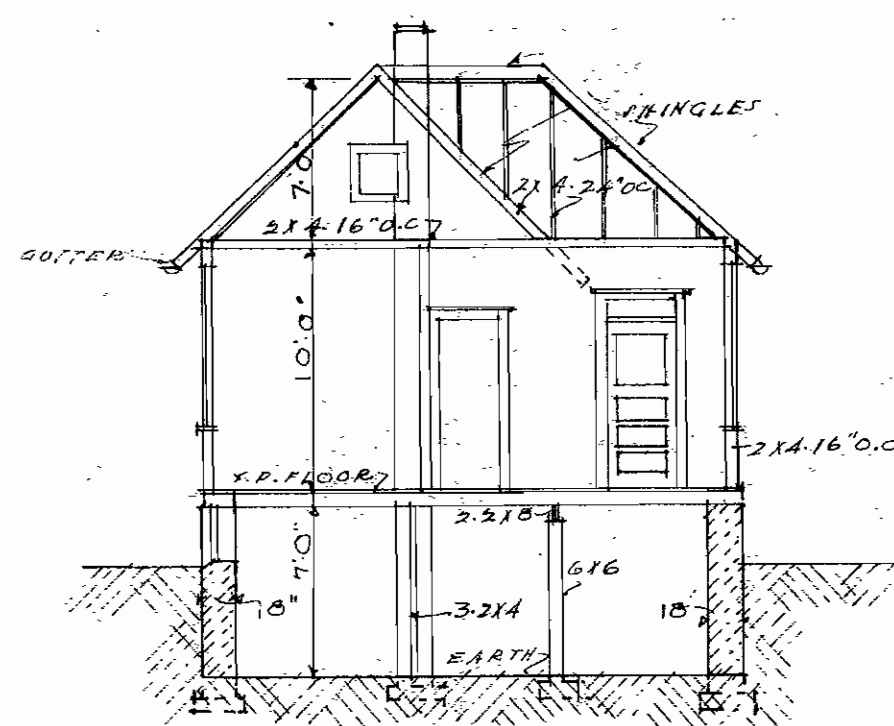
SECTION
